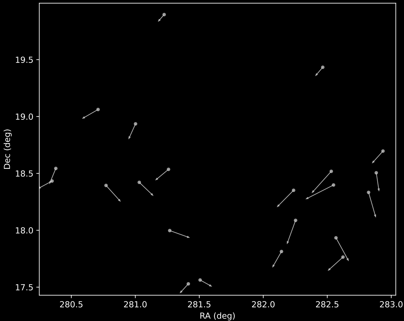
APOGEE DR17 Cluster 15 Proper Motion Vectors (n=22)
