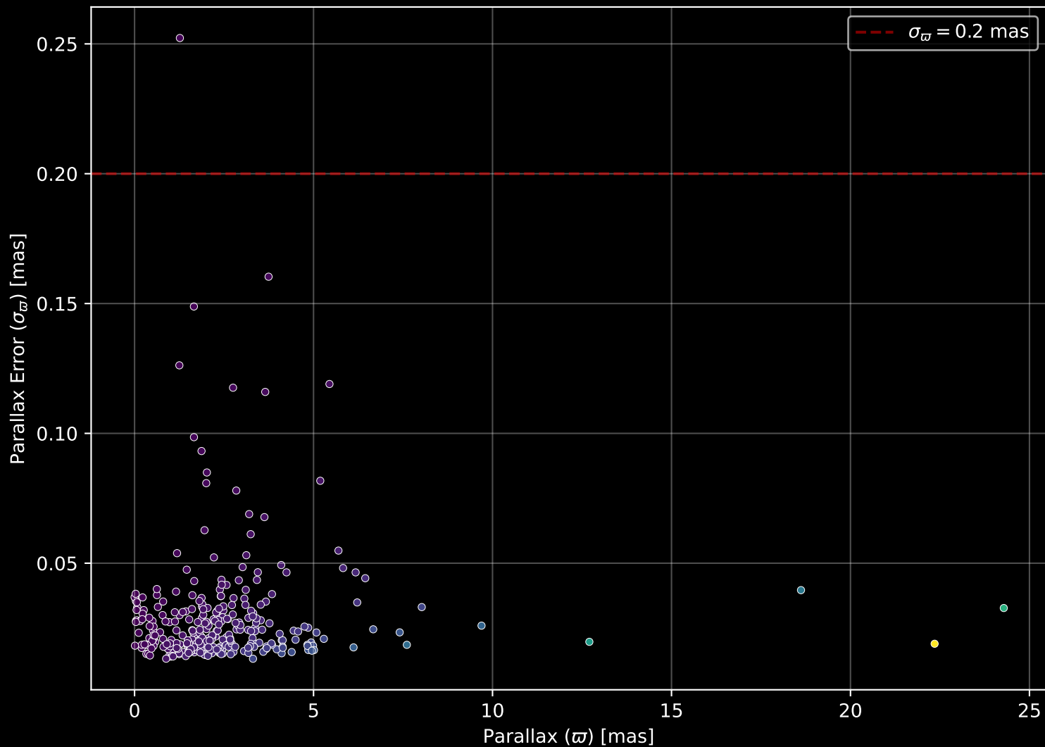
APOGEE DR17 Field: [N4147] Parallax Quality (n= 307)
