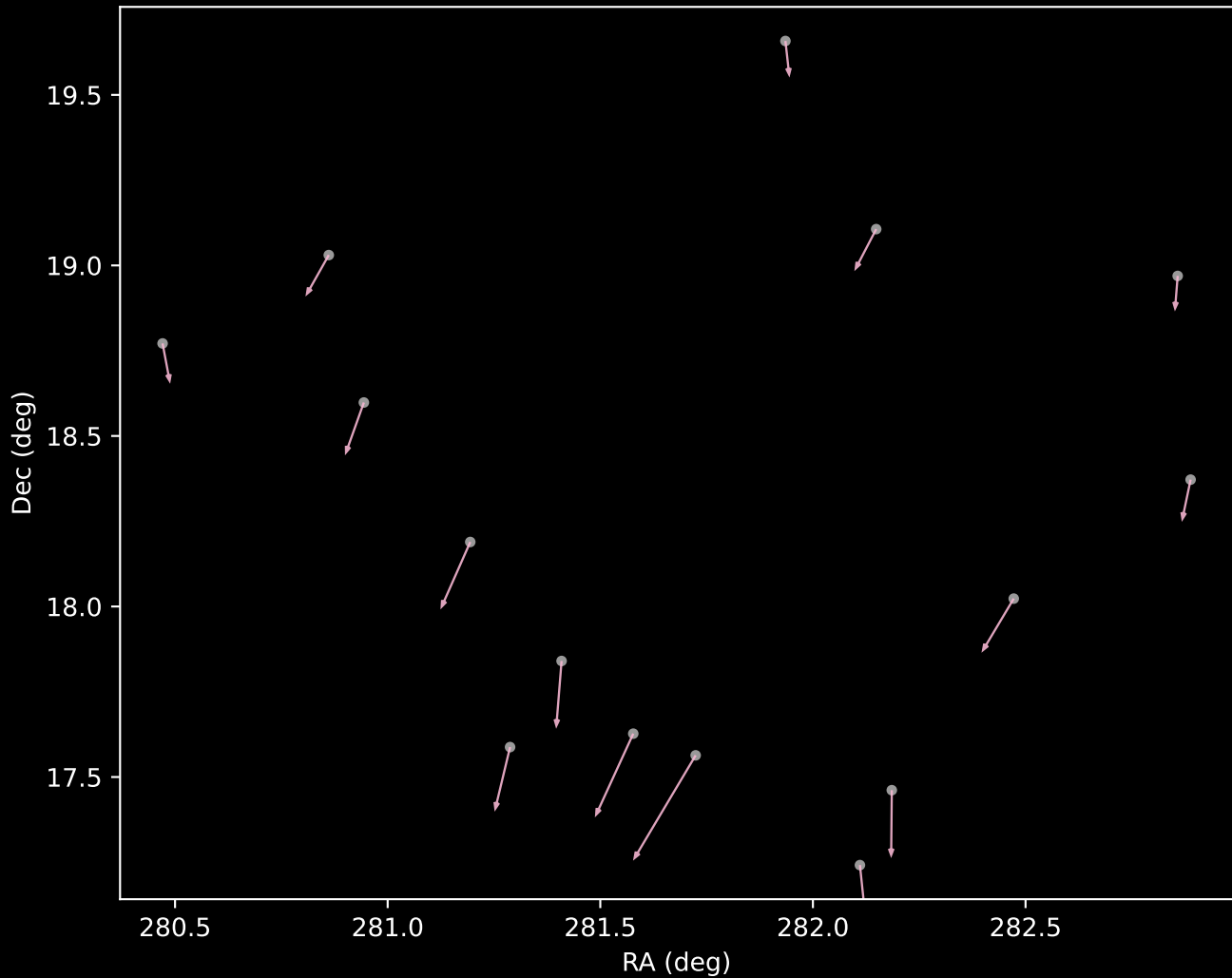
APOGEE DR17 Cluster 13 Proper Motion Vectors (n=15)
