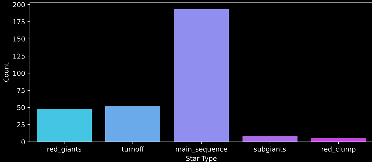
APOGEE DR17 Field: [N4147] Count plot of Star Type
