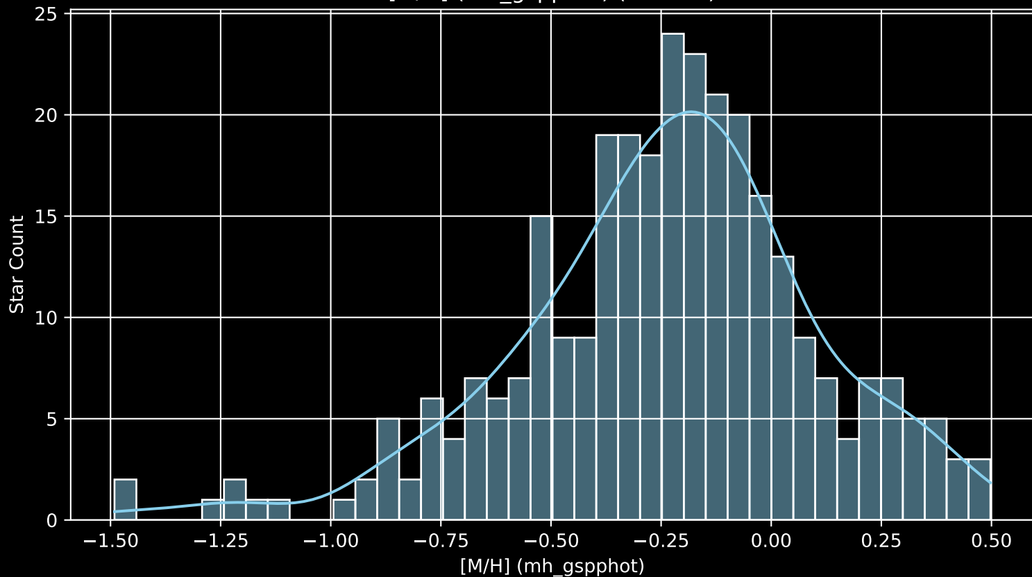
APOGEE DR17 Field: [N4147 [M/H] (mh_gspphot) (n= 303)
