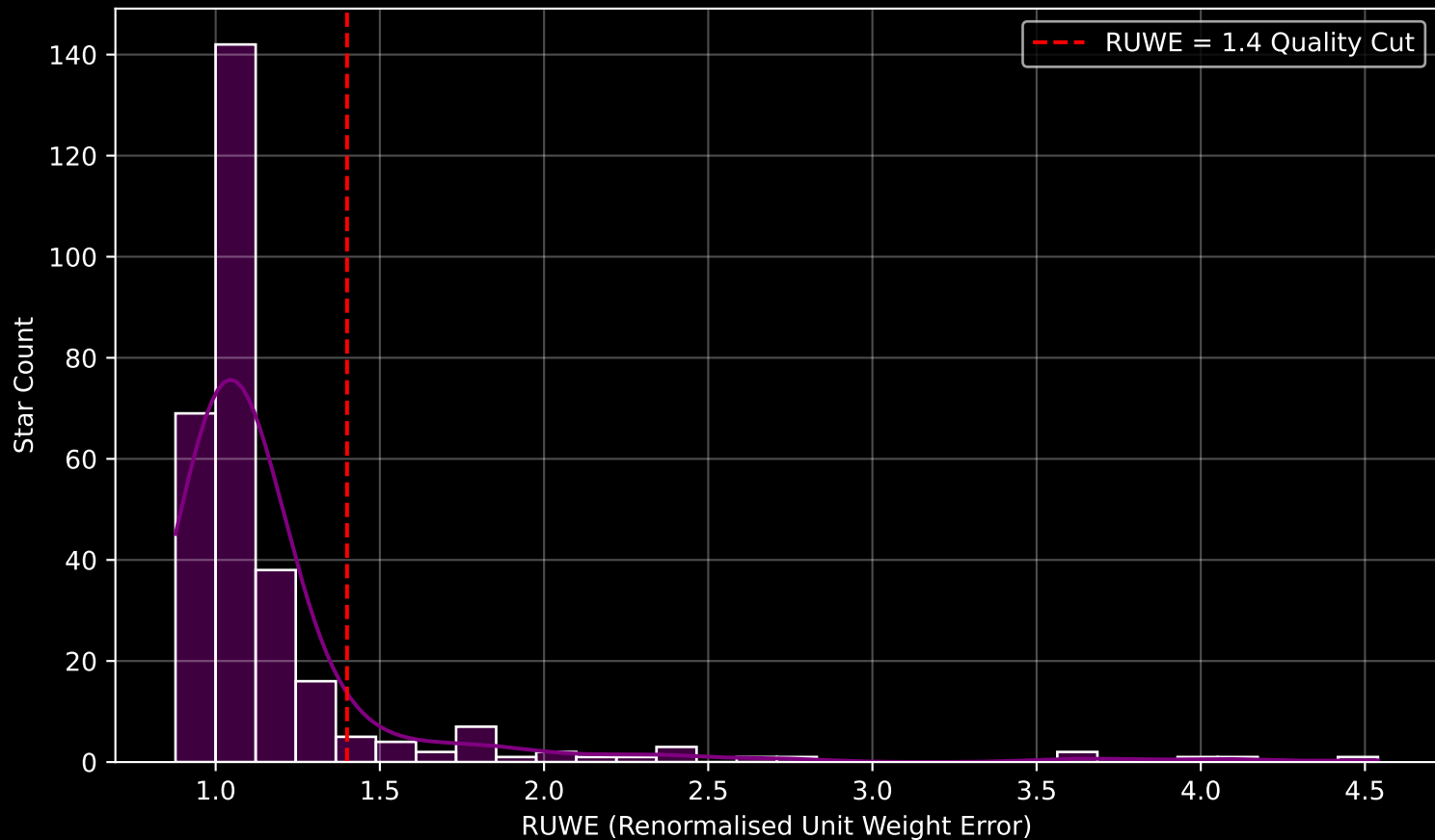
GAPOGEE DR17 Field [N4147] RUWE Distribution (n= 298)
