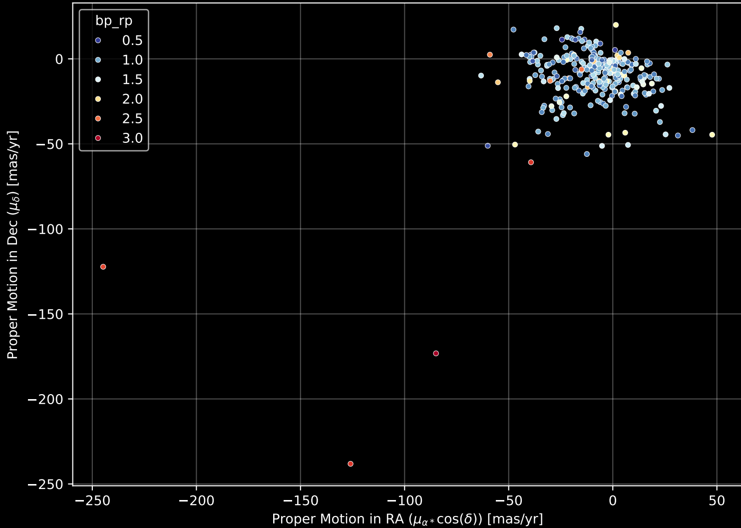
APOGEE DR17 Field: [N4147] Proper Motion Diagram (n= 307)
